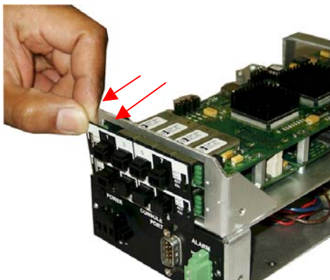
Figure 3.6.1d: Removing PM screen Plate
